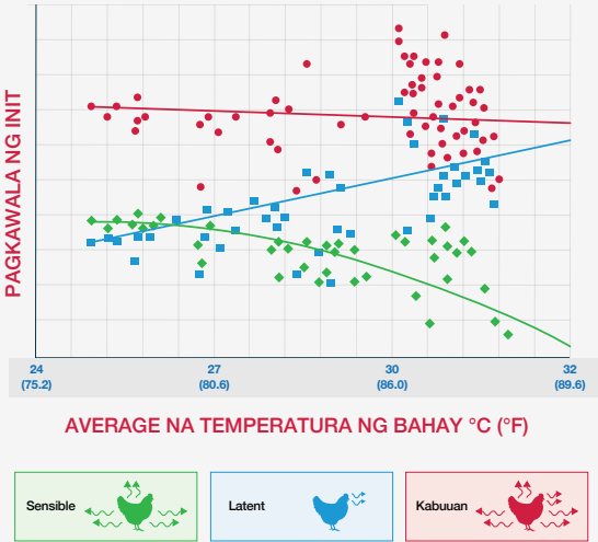
Sensible at latent heat loss.
