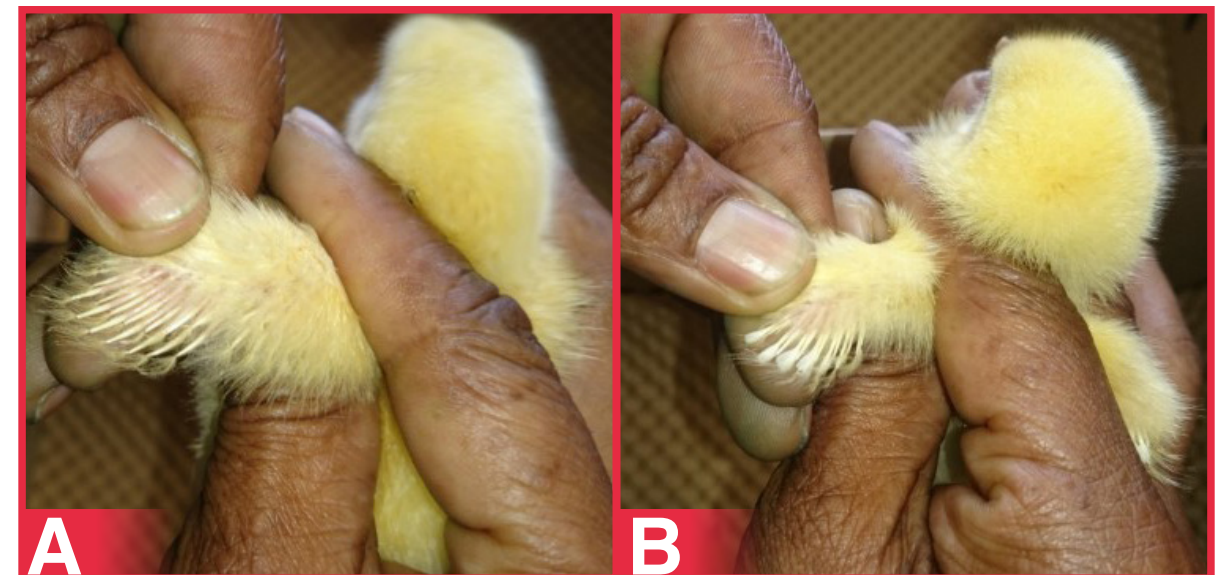
Figure 5. Day-old chicks showing the natal down and the initial appearance of the first phase feathers. The left hand chick (A) carries the fast-feathering gene (k) and the right hand chick (B) the slow-feathering gene (K).
